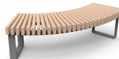
3-place curved bench Inner diameter Ø 2.12 m External diameter Ø 3.06 m Ref. 10 3460
